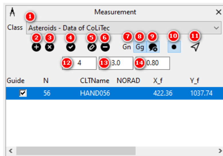
Figure 13. Manual measurement window functions
