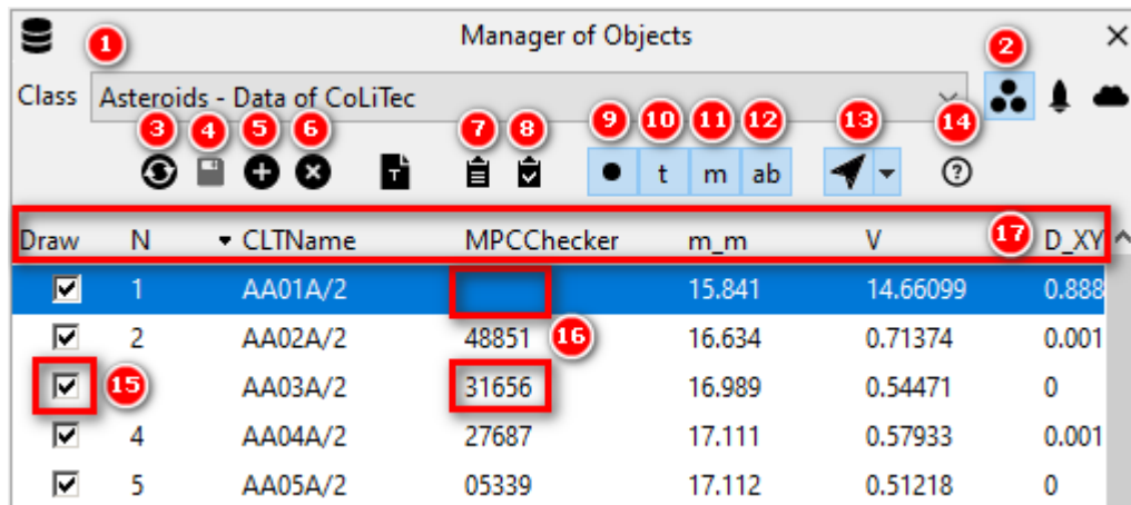
Figure 8. Manager of Objects features
