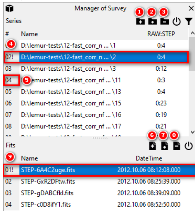
Figure 5. Manager of Survey
